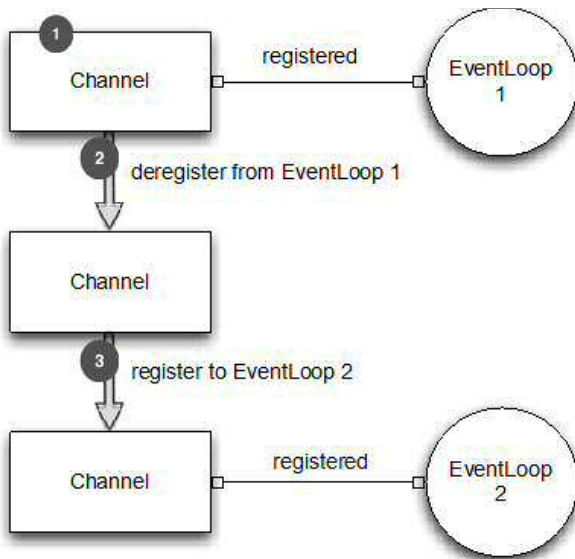
Figure 16.3 Migrate a Channel from one EventLoop to another
