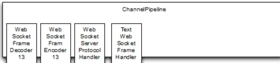
Figure 11.4 Server logic
