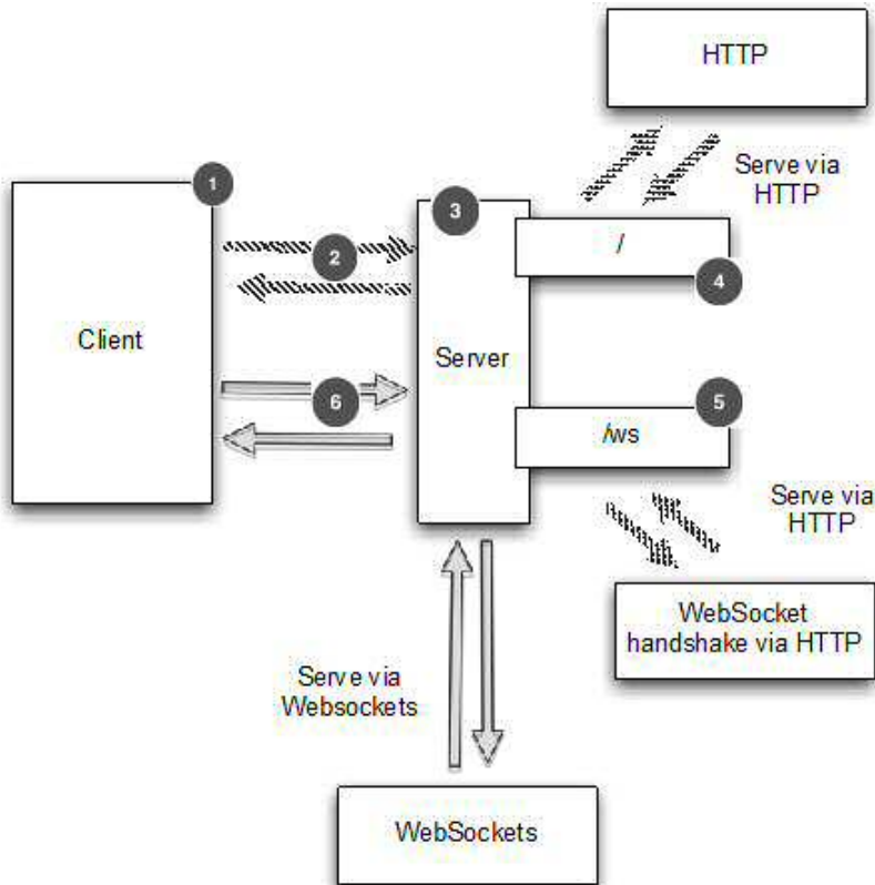
Figure 11.2 Server logic
