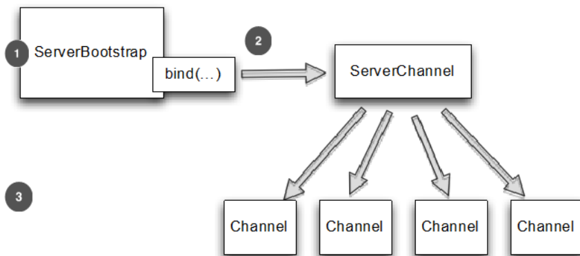
Figure 9.3 ServerBootstrap
