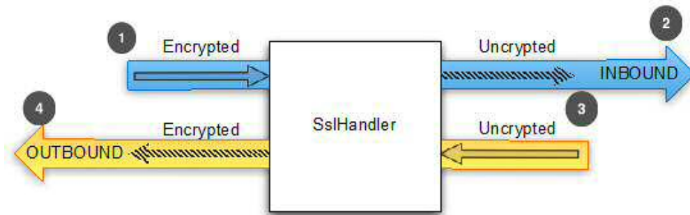
Figure 8.1 SslHandler
