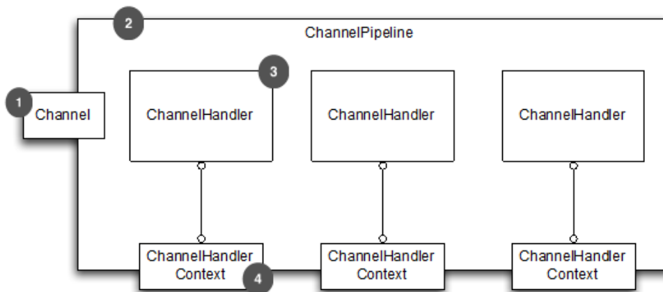
Figure 6.2 ChannelPipeline , ChannelHandlerContext and Channel
