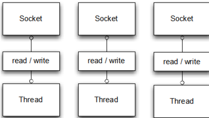
Figure 1.2 Blocking IO
