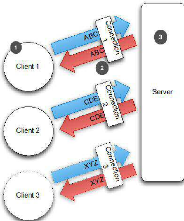
Figure 2.1 Application overview
