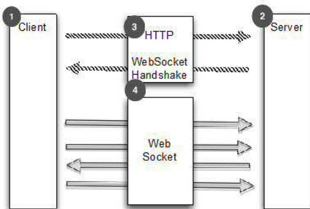
Figure 8.4 WebSocket
