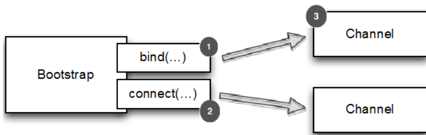
Figure 9.2 Bootstrap
