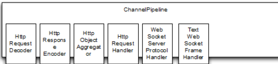
Figure 11.3 Server logic
