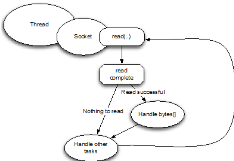
Figure 4.3 OIO-Processing logic
